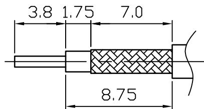
Recommended Cable Stripping Dimensions
