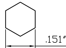
Recommended Crimped Dimensions For Ferrule
